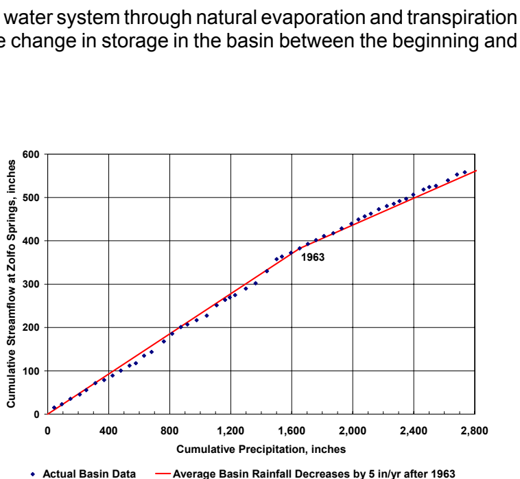
Figure 4 Accumulated Annual Streamflow for Peace River at Zolfo Springs versus Accumulated Annual Rainfall at Bartow, 1934 - 1984.
