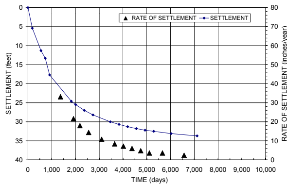
Figure 17. Settlement and Rate of Settlement vs Time for Typical Clay Settling Area.
