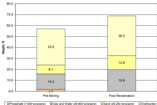
Figure 14. Comparison of Average Thickness of Soil Profile Before and After Mining.
