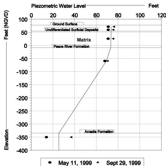
Figure 11. Piezometric Levels versus Depth for Typical Cluster Wells near Ona, Hardee County, Florida.
