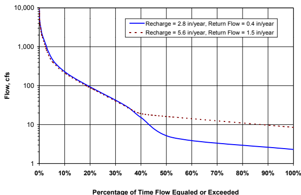
Figure 18. Effect of Increasing Deep Recharge on Flow-Duration Curve for Hypothetical Watershed.
