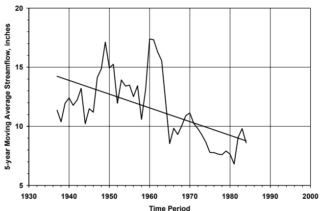
Figure 2. 5-year Moving Average Streamflow in Peace River at Arcadia
