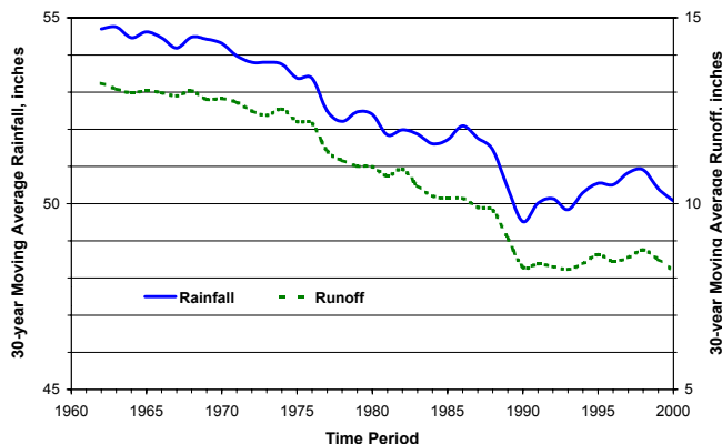
Figure 5. 30-year Moving Average Rainfall and Runoff in Peace River Basin.
