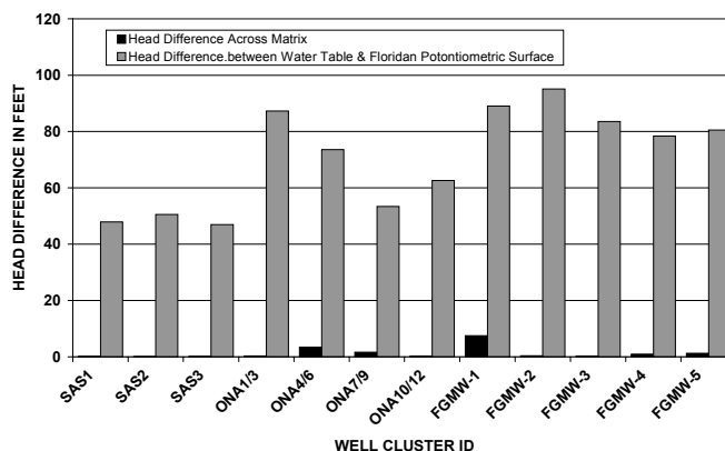
Figure 12. Comparison of Head Difference Across Matrix with Head Difference between Surficial and Floridan Aquifers.
