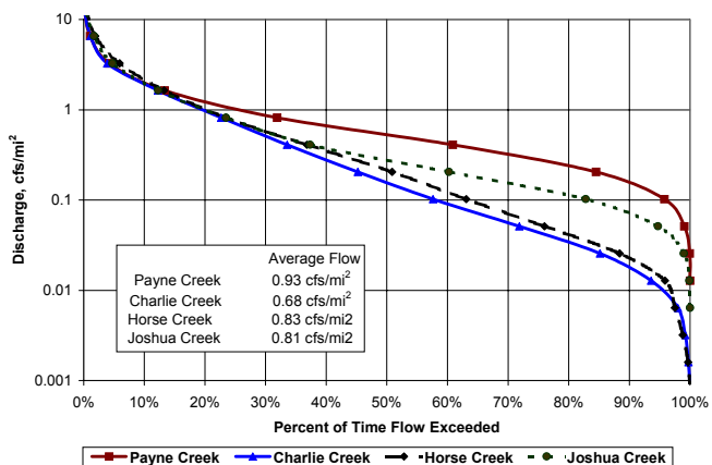
Figure 13. Comparison of Flow-Duration Curves for Mined and Unmined Creeks in the Peace River Basin.
