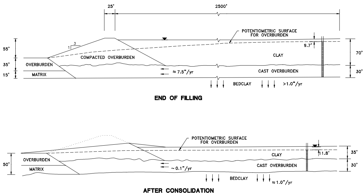
Figure 15. Cross Section through Clay Settling Area
