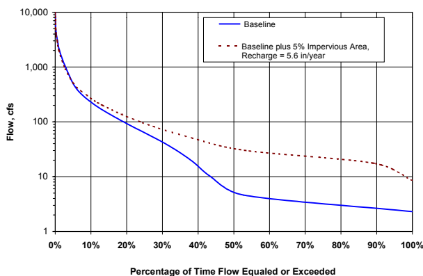
Figure 20. Effect of Adding 5 Percent Impervious Area and Doubling Deep Recharge on Duration Curve for Hypothetical watershed.
