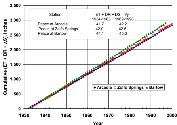
Figure 8. Accumulated difference between Rainfall and Streamflow for Peace River at Arcadia, Bartow, and Zolfo Springs.
