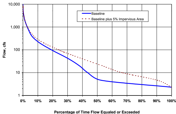
Figure 19. Effect of Adding 5 Percent Impervious Area on Flow-Duration Curve for Hypothetical Watershed.
