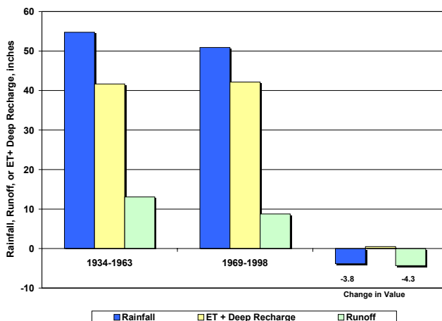
Figure 7. Water Budget for Peace River at Arcadia for Historic and Recent 30-year Periods.
