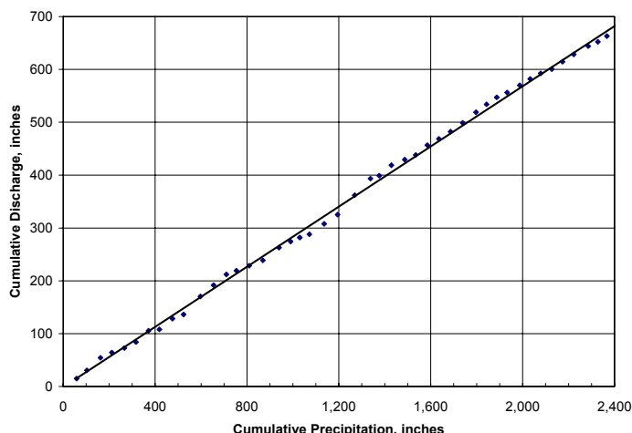
Figure 3. Accumulated Annual Streamflow for Myakka River at Sarasota versus Accumulated Annual Rainfall at Bartow.
