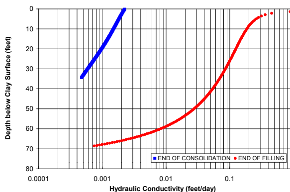
Figure 16. Hydraulic Conductivity versus Depth for Typical clay Settling Area.
